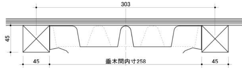
@303垂木高さ45
