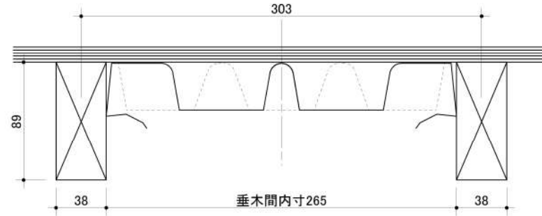
@303垂木高さ89
